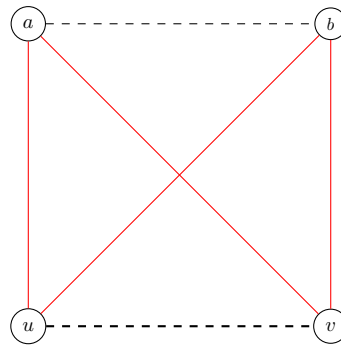
Figure 4: If u and v are from the same component in \overline{G} , but a and b do not belong to this component, then these four vertices form a 4-cycle in G . The dotted lines represent edges that may or may not exist and the solid red lines show the edges that form a 4-cycle in G .
