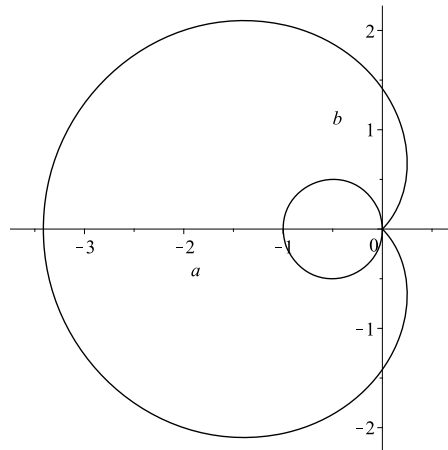
Figure 11: The limits of roots of A(K_{1,n-1}[K_2], x) .
