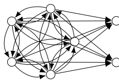
Figure 5: F(K_5 \overrightarrow{\vee} K_2) = 5 and Z(K_5 \overrightarrow{\vee} K_2) = 6 .
